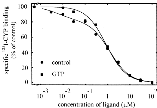
Figure 2. Competition curve of Broxaterol for ^{125}\text{I} -CYP binding to \beta_2 -receptors without (●) and in the presence (■) of 100\text{ }\mu\text{M} GTP.
