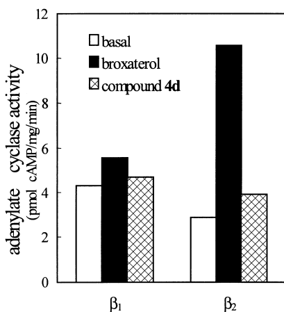
Figure 3. Activity of adenylate cyclase mediated by the stimulation of \beta_1 - and \beta_2 -adrenergic receptors.
